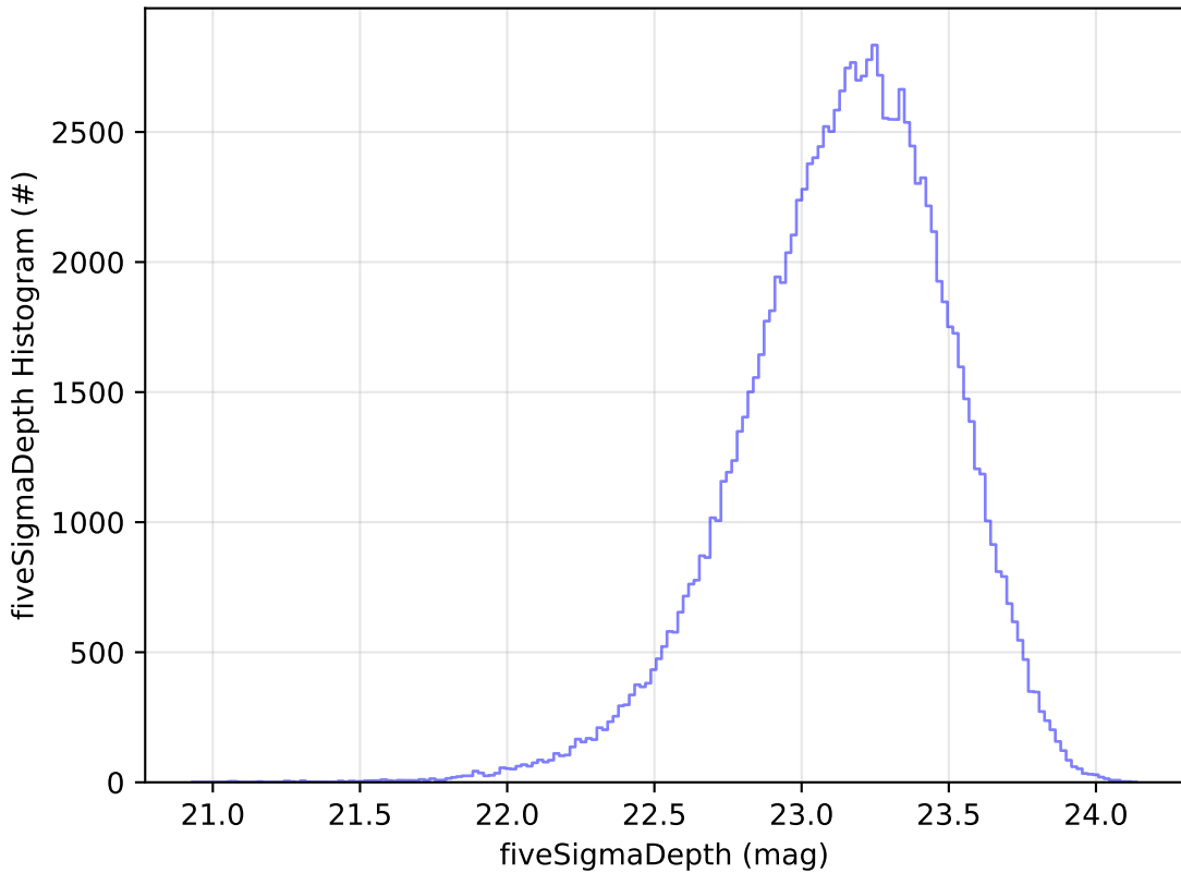
roll_uniform_early_half_mjdp67_v3.4_10yrs u: fiveSigmaDepth Histogram
