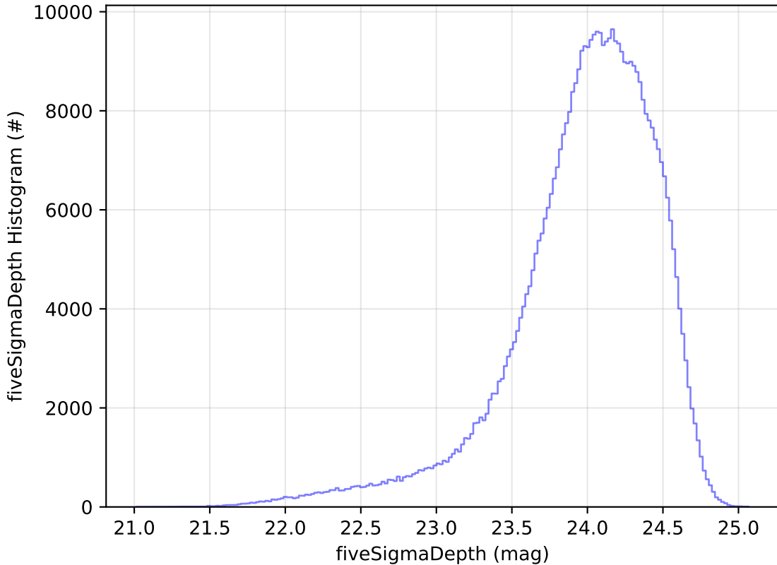
roll_uniform_early_half_mjdp67_v3.4_10yrs r: fiveSigmaDepth Histogram
