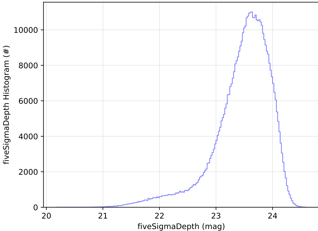
roll_uniform_early_half_mjdp67_v3.4_10yrs i: fiveSigmaDepth Histogram
