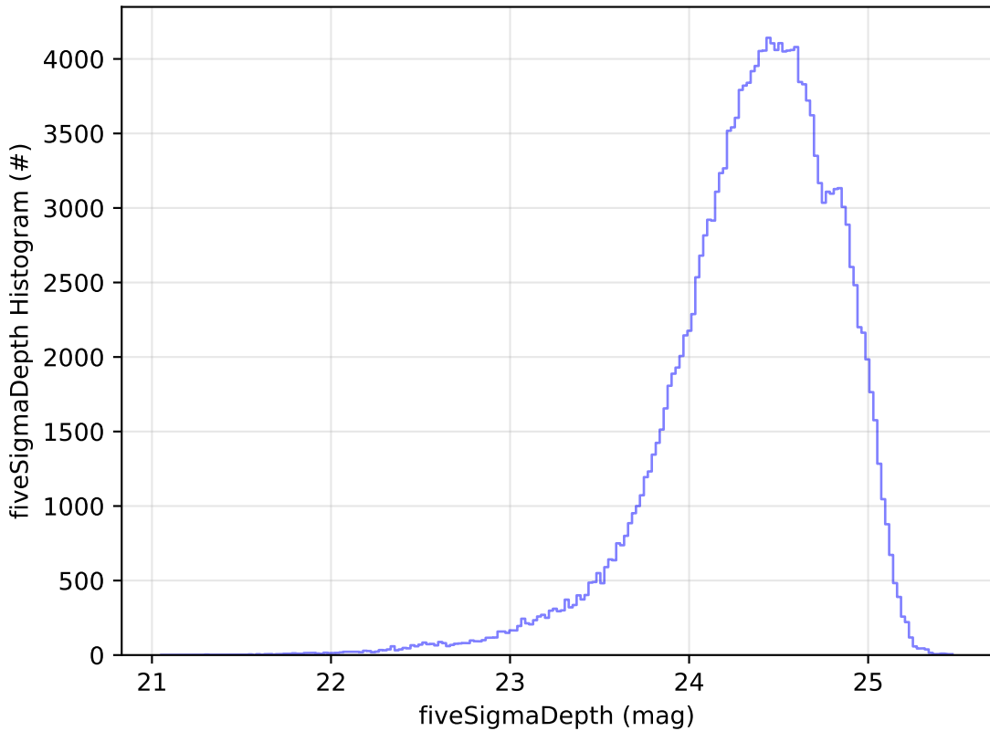
roll_uniform_early_half_mjdp67_v3.4_10yrs g: fiveSigmaDepth Histogram
