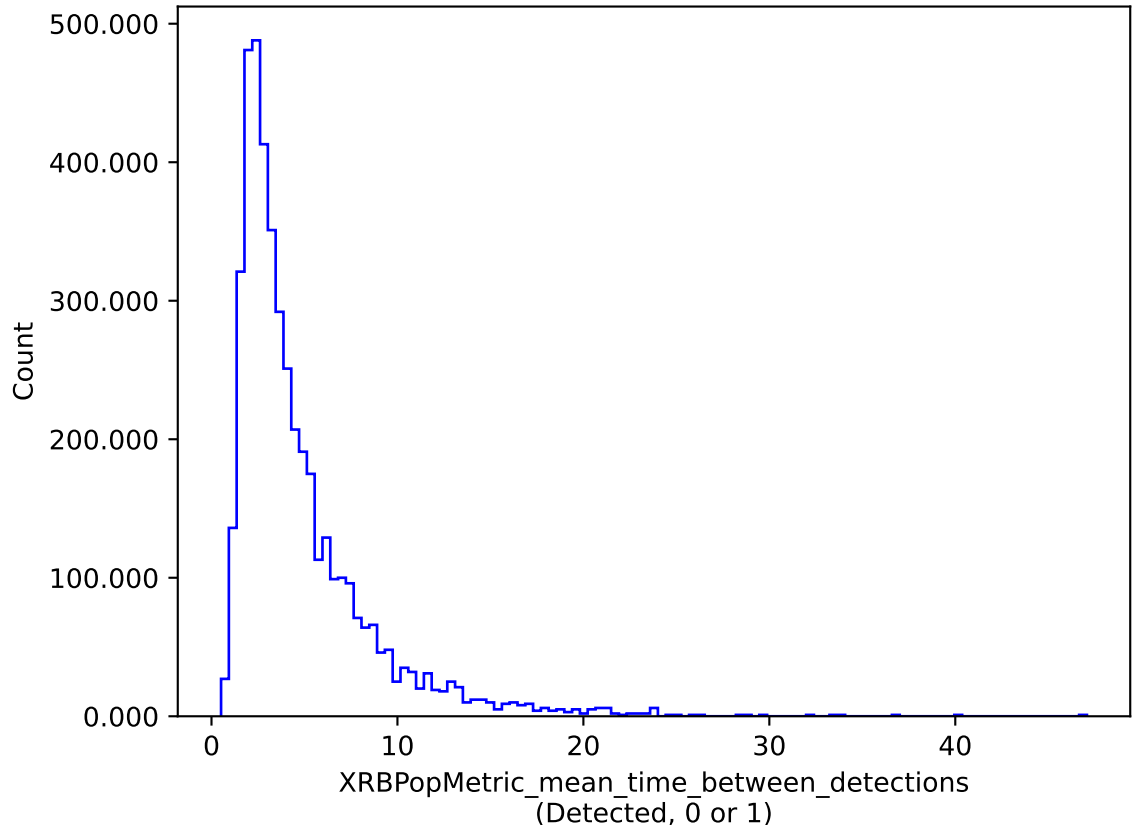
roll_uniform_early_half_mjdp67_v3.4_10yrs : XRBPoMetric_mean_time_between_detections
