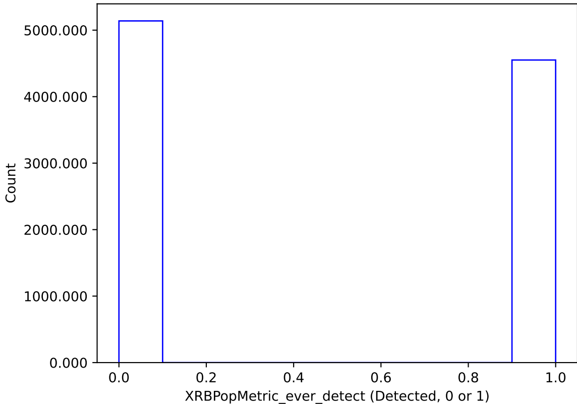
roll_uniform_early_half_mjdp67_v3.4_10yrs : XRBPopMetric_ever_detect
