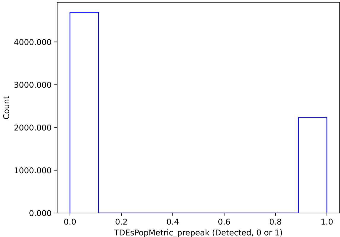
roll_uniform_early_half_mjdp67_v3.4_10yrs : TDEsPopMetric_prepeak
