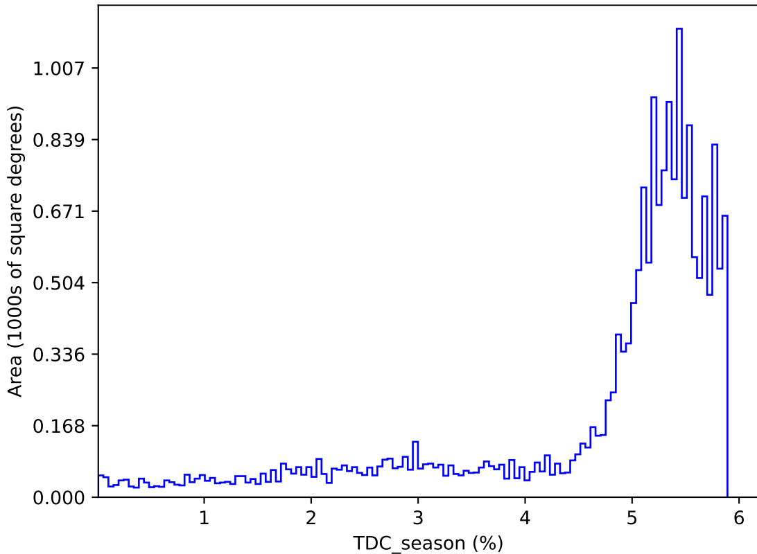
roll_uniform_early_half_mjdp67_v3.4_10yrs : TDC_season
