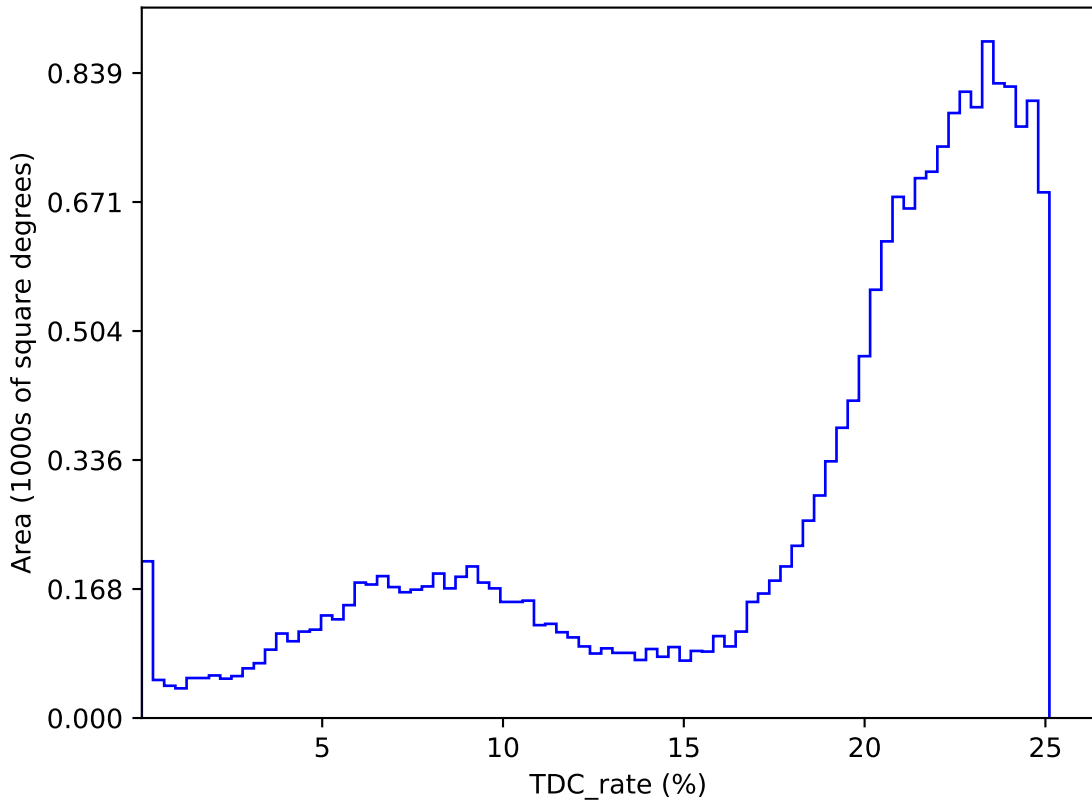
roll_uniform_early_half_mjdp67_v3.4_10yrs : TDC_rate
