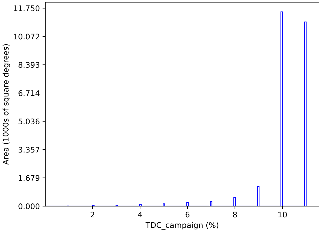
roll_uniform_early_half_mjdp67_v3.4_10yrs : TDC_campaign
