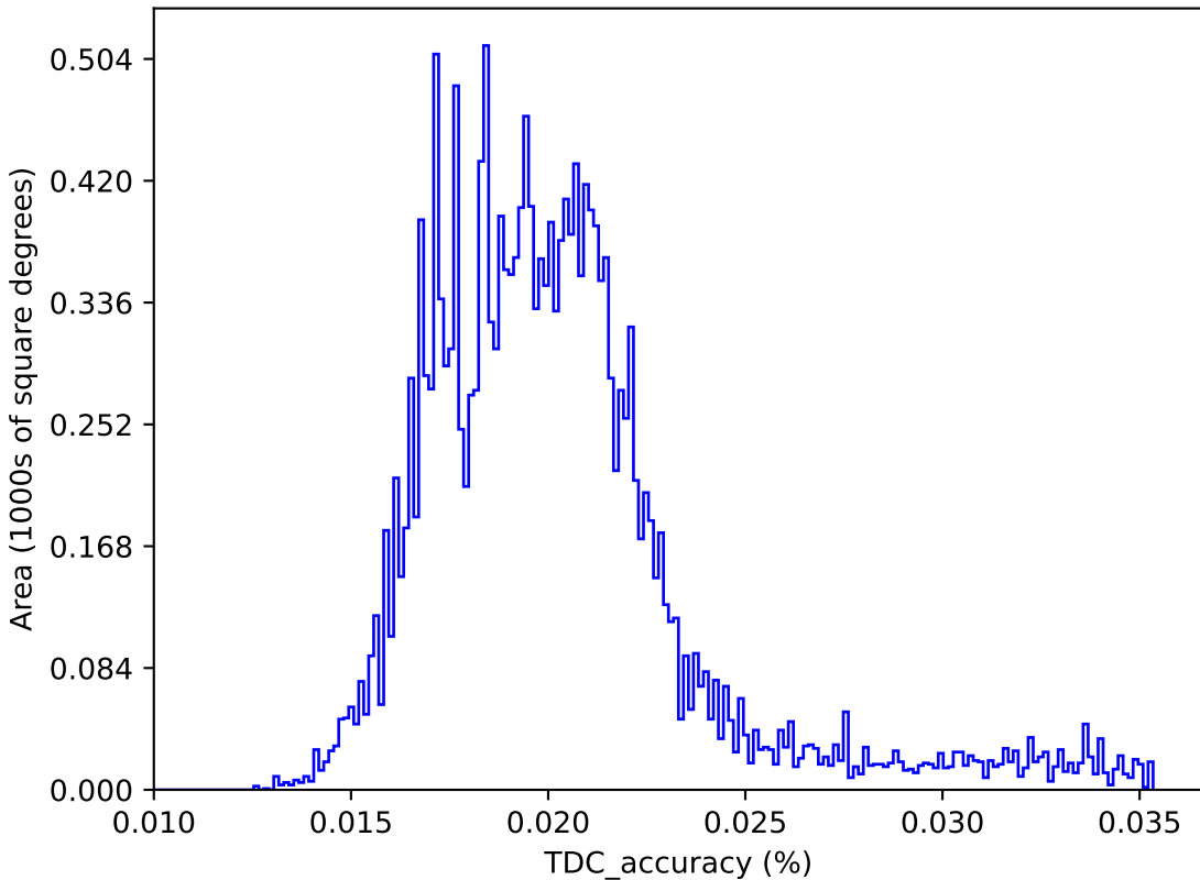
roll_uniform_early_half_mjdp67_v3.4_10yrs : TDC_accuracy
