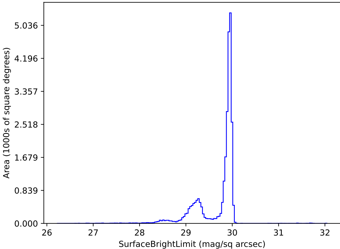
roll_uniform_early_half_mjdp67_v3.4_10yrs i: SurfaceBrightLimit
