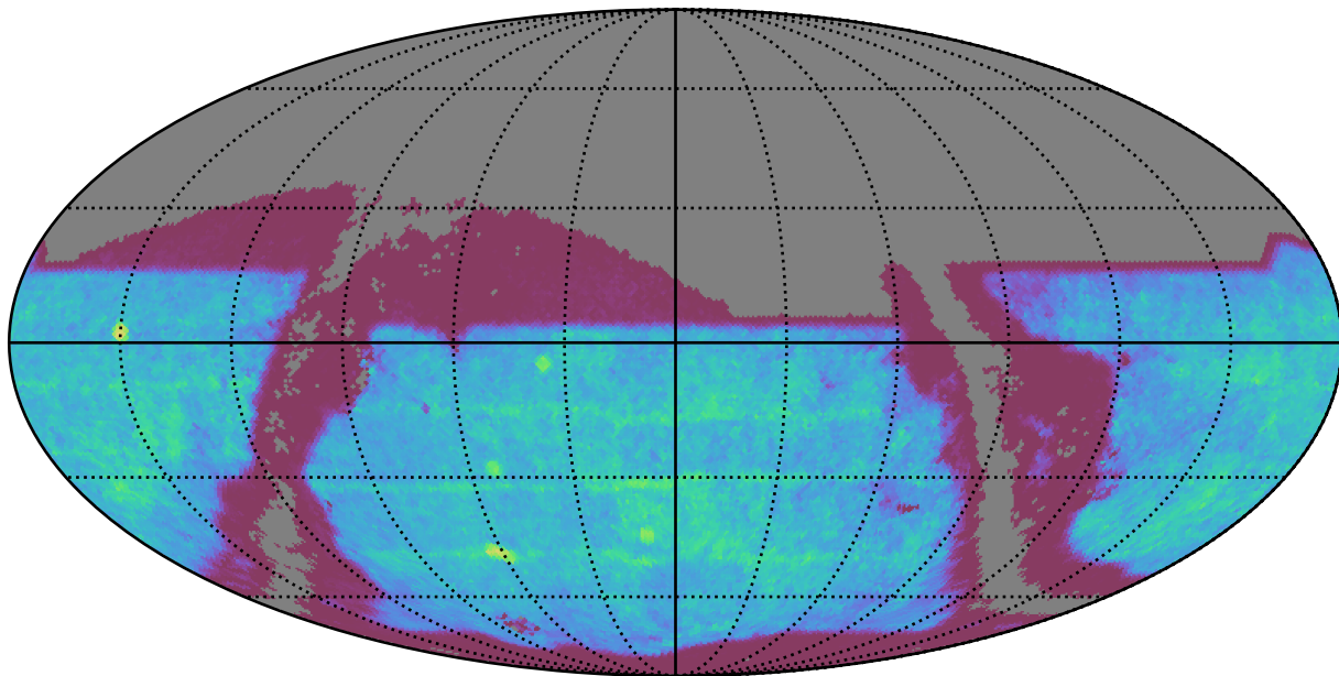
roll_uniform_early_half_mjdp67_v3.4_10yrs : SNSLMetric
