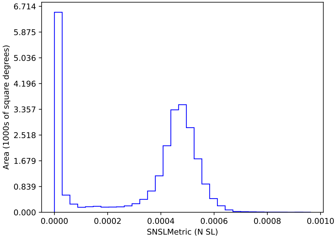
roll_uniform_early_half_mjdp67_v3.4_10yrs : SNSLMetric
