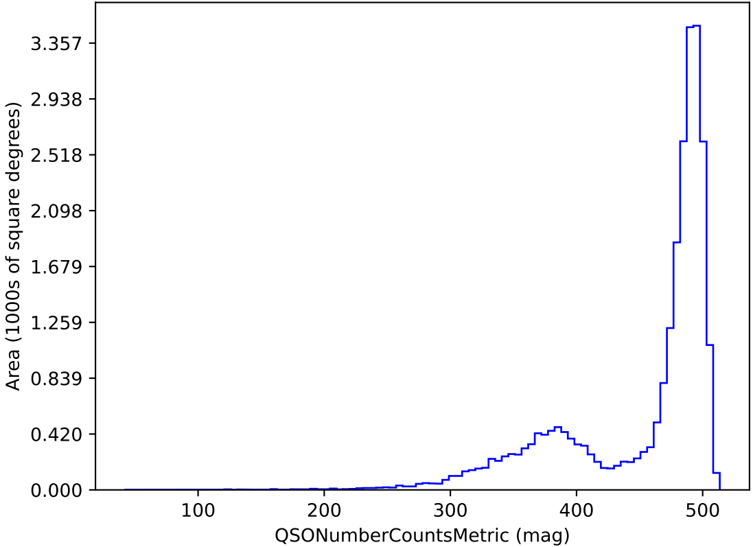
roll_uniform_early_half_mjdp67_v3.4_10yrs z band and non-DD: QSONumberCountsMetric
