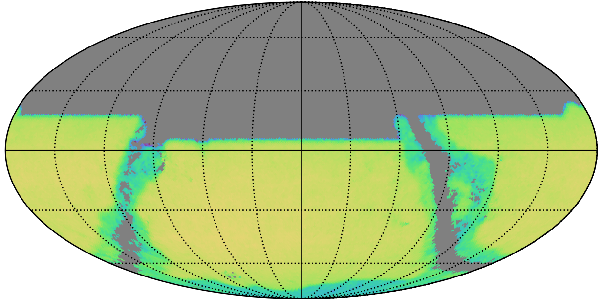
roll_uniform_early_half_mjdp67_v3.4_10yrs y band and non-DD: QSONumberCountsMetric
