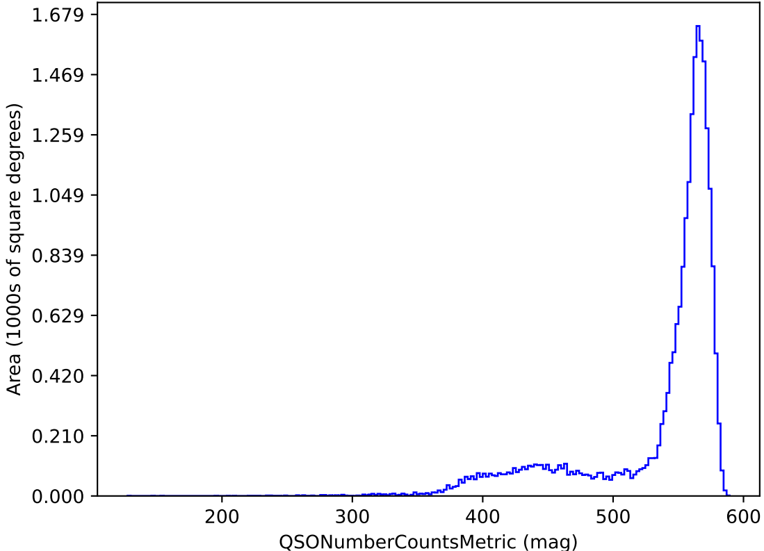
roll_uniform_early_half_mjdp67_v3.4_10yrs y band and non-DD: QSONumberCountsMetric
