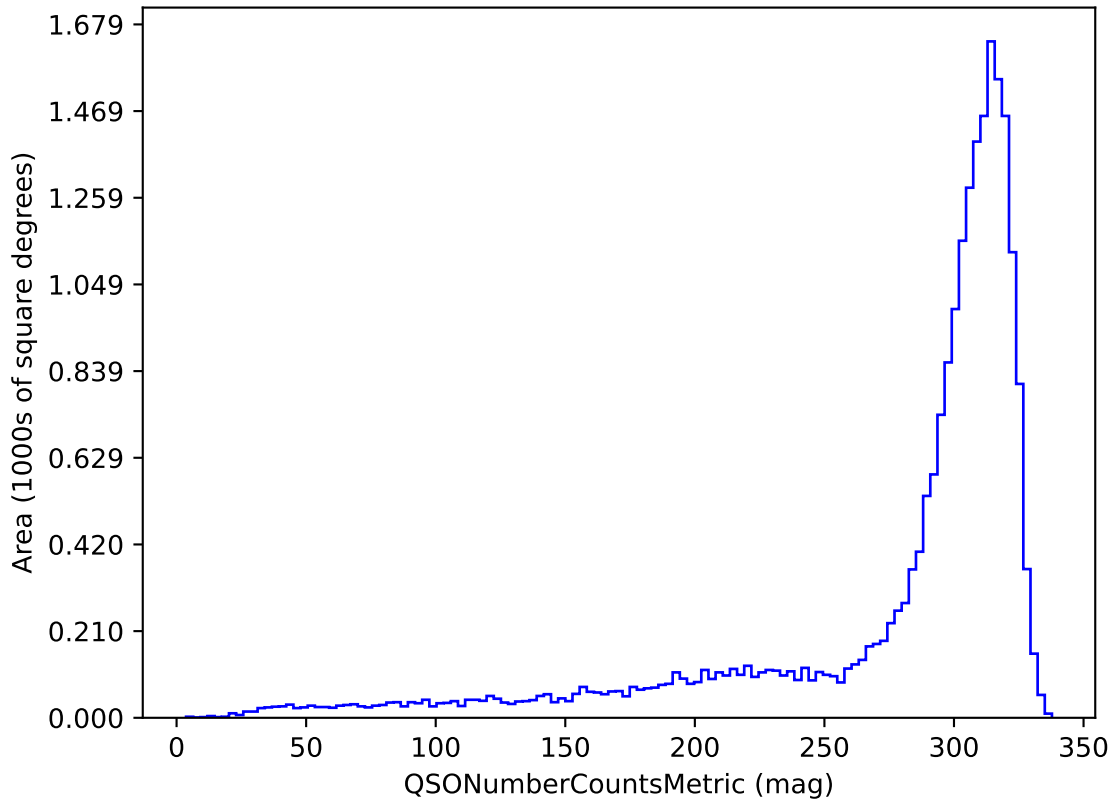
roll_uniform_early_half_mjdp67_v3.4_10yrs u band and non-DD: QSONumberCountsMetric
