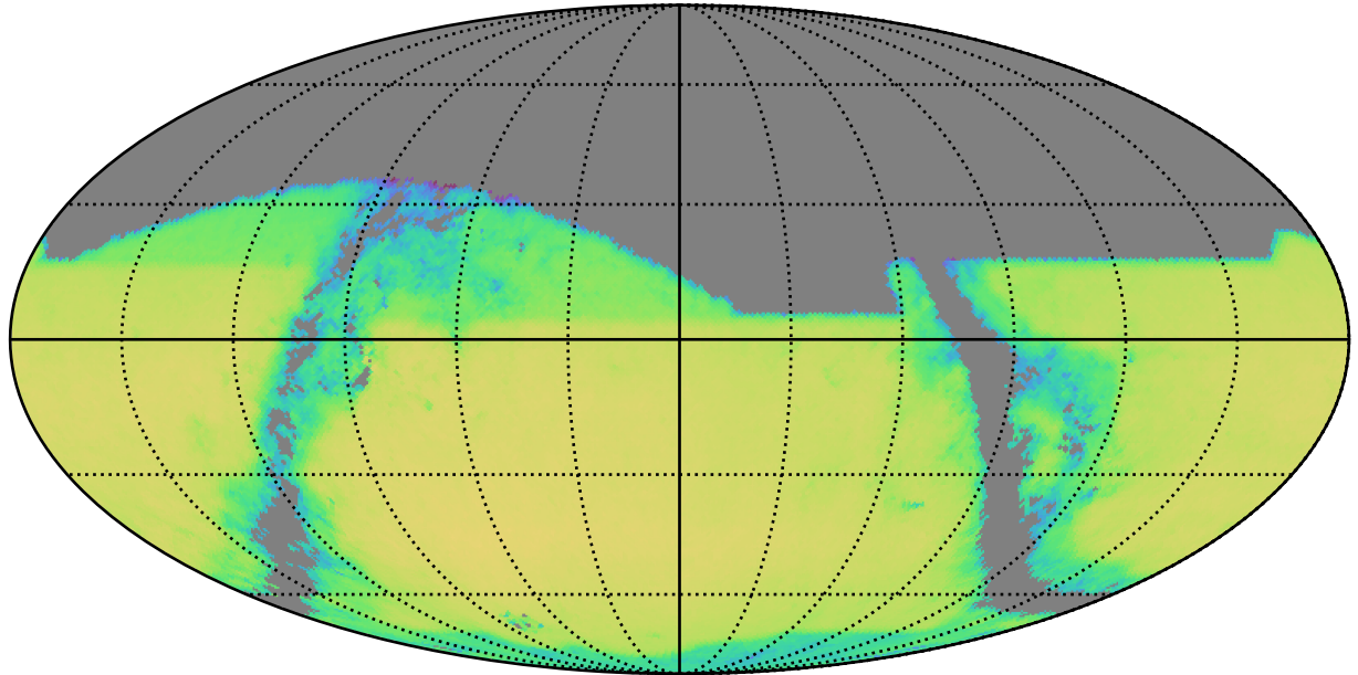
roll_uniform_early_half_mjdp67_v3.4_10yrs r band and non-DD: QSONumberCountsMetric
