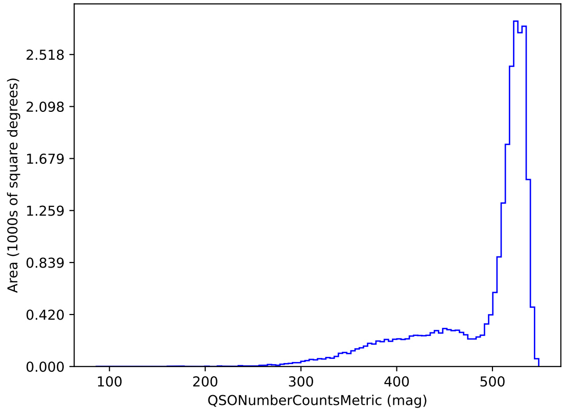
roll_uniform_early_half_mjdp67_v3.4_10yrs r band and non-DD: QSONumberCountsMetric
