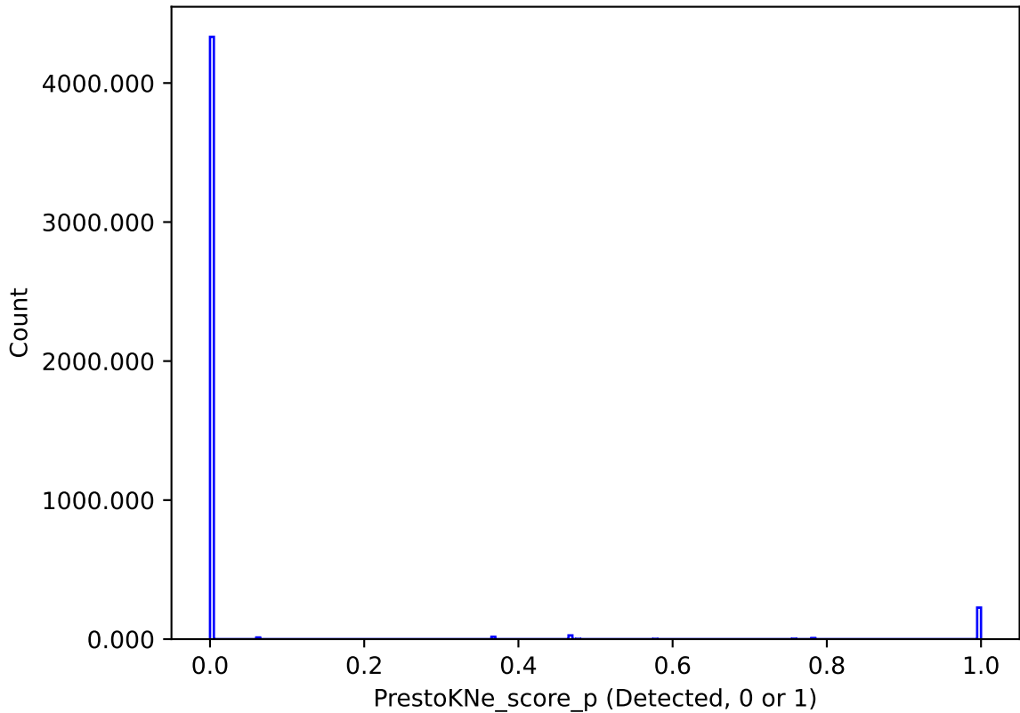
roll_uniform_early_half_mjdp67_v3.4_10yrs : PrestoKNe_score_p
