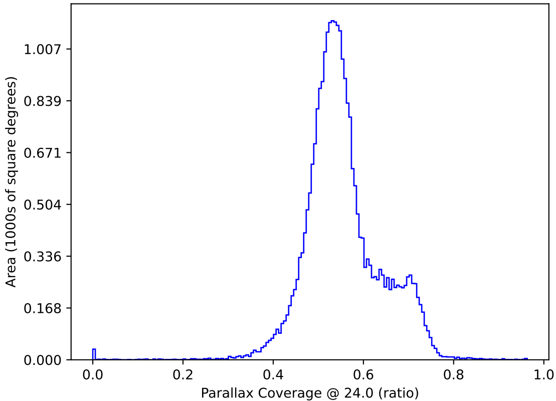
roll_uniform_early_half_mjdp67_v3.4_10yrs : Parallax Coverage @ 24.0
