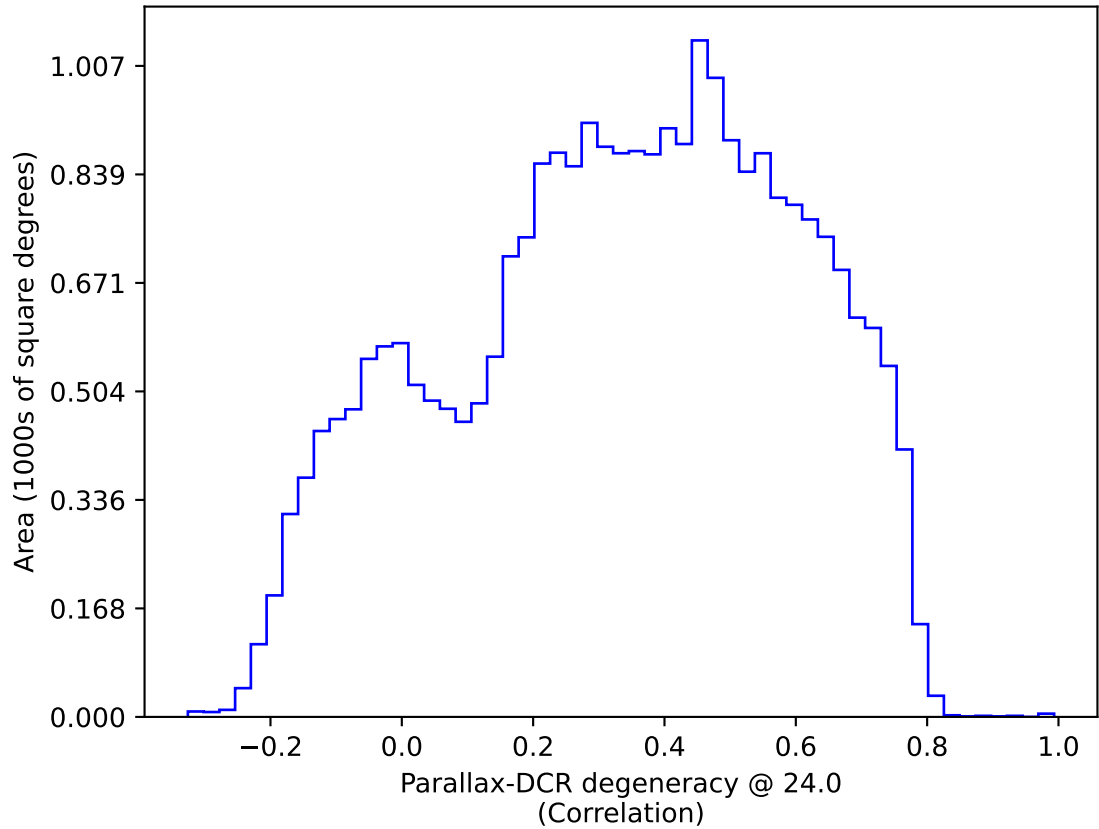
roll_uniform_early_half_mjdp67_v3.4_10yrs : Parallax-DCR degeneracy @ 24.0
