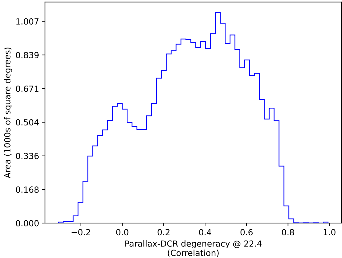
roll_uniform_early_half_mjdp67_v3.4_10yrs : Parallax-DCR degeneracy @ 22.4
