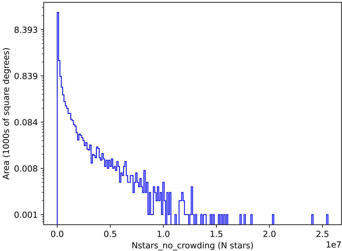
roll_uniform_early_half_mjdp67_v3.4_10yrs y: Nstars_no_crowding
