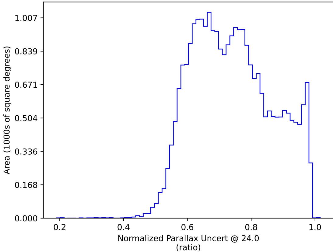
roll_uniform_early_half_mjdp67_v3.4_10yrs : Normalized Parallax Uncert @ 24.0
