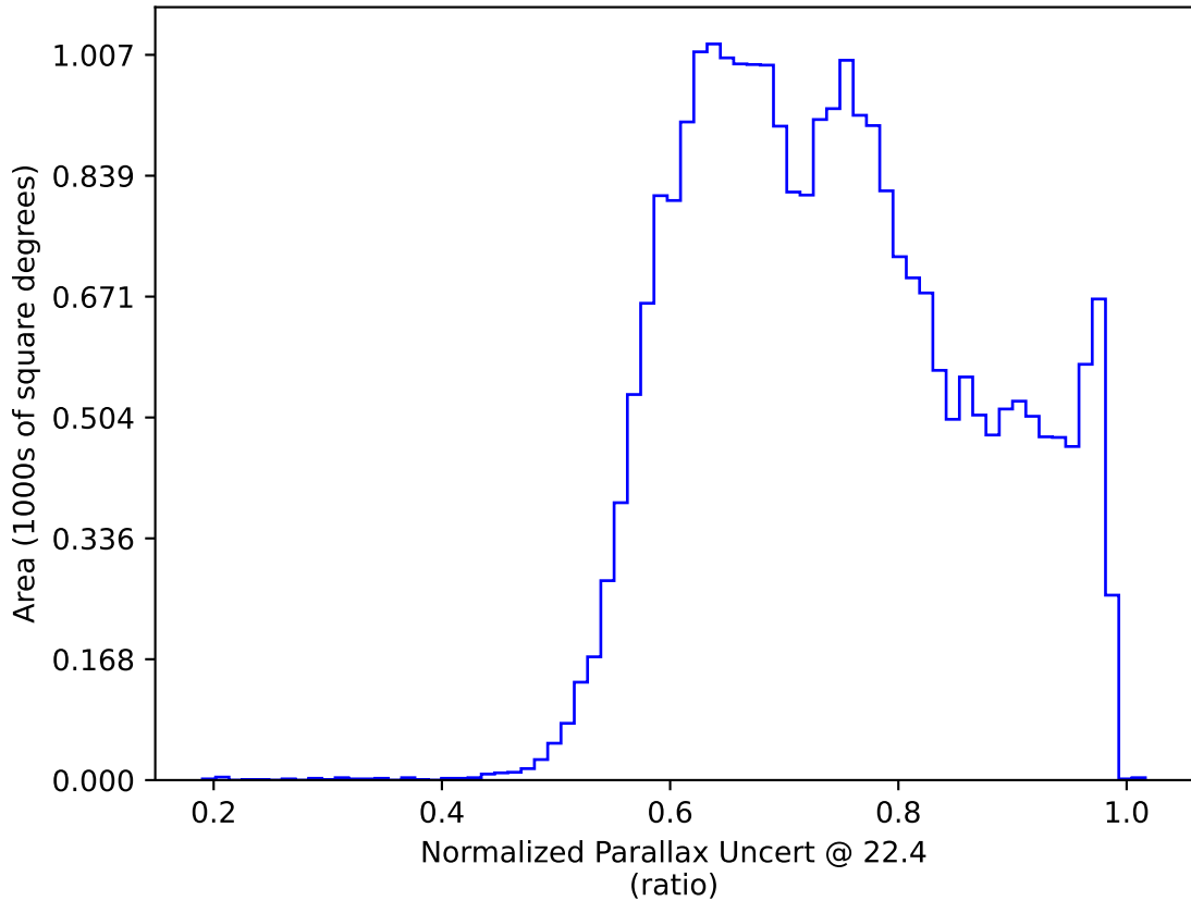
roll_uniform_early_half_mjdp67_v3.4_10yrs : Normalized Parallax Uncert @ 22.4
