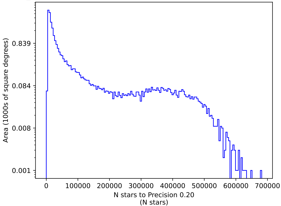
roll_uniform_early_half_mjdp67_v3.4_10yrs r: N stars to Precision 0.20
