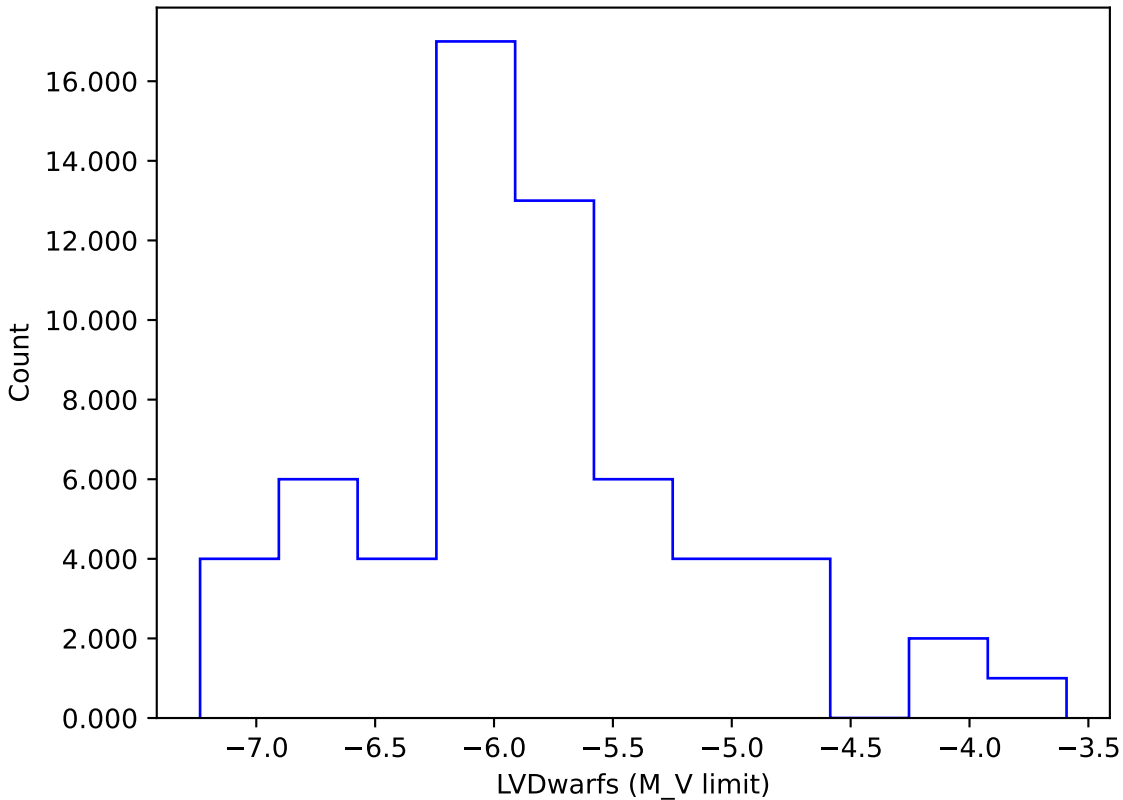
roll_uniform_early_half_mjdp67_v3.4_10yrs gi: LVDwarfs
