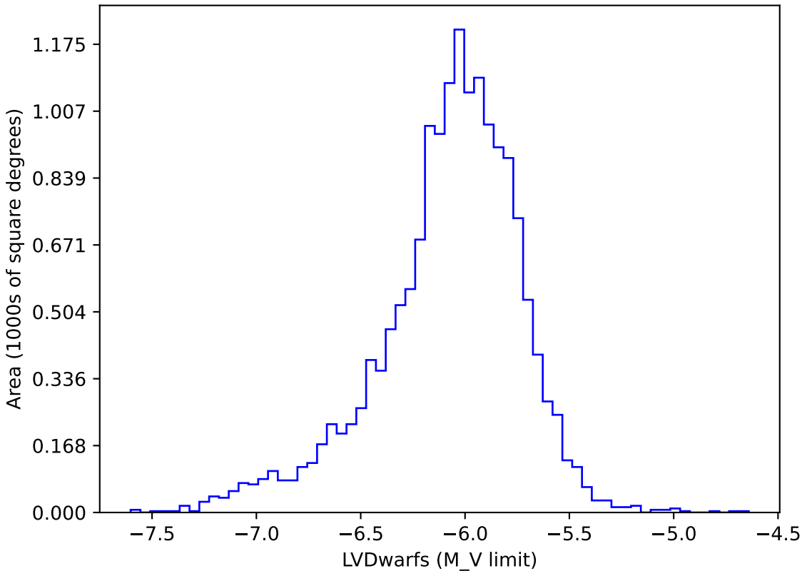
roll_uniform_early_half_mjdp67_v3.4_10yrs gi: LVDwarfs
