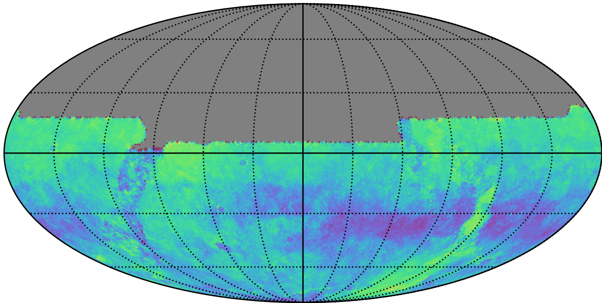
roll_uniform_early_half_mjdp67_v3.4_10yrs u: Kuiper rotSkyPos
