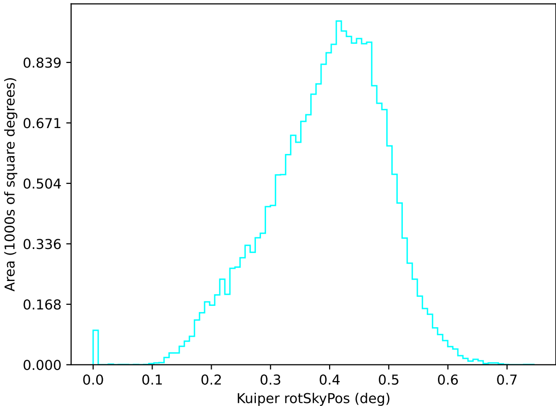
roll_uniform_early_half_mjdp67_v3.4_10yrs u: Kuiper rotSkyPos
