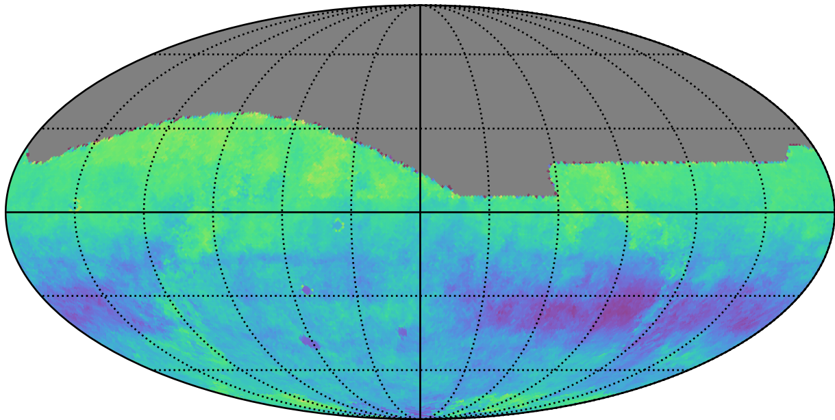
roll_uniform_early_half_mjdp67_v3.4_10yrs r: Kuiper rotSkyPos
