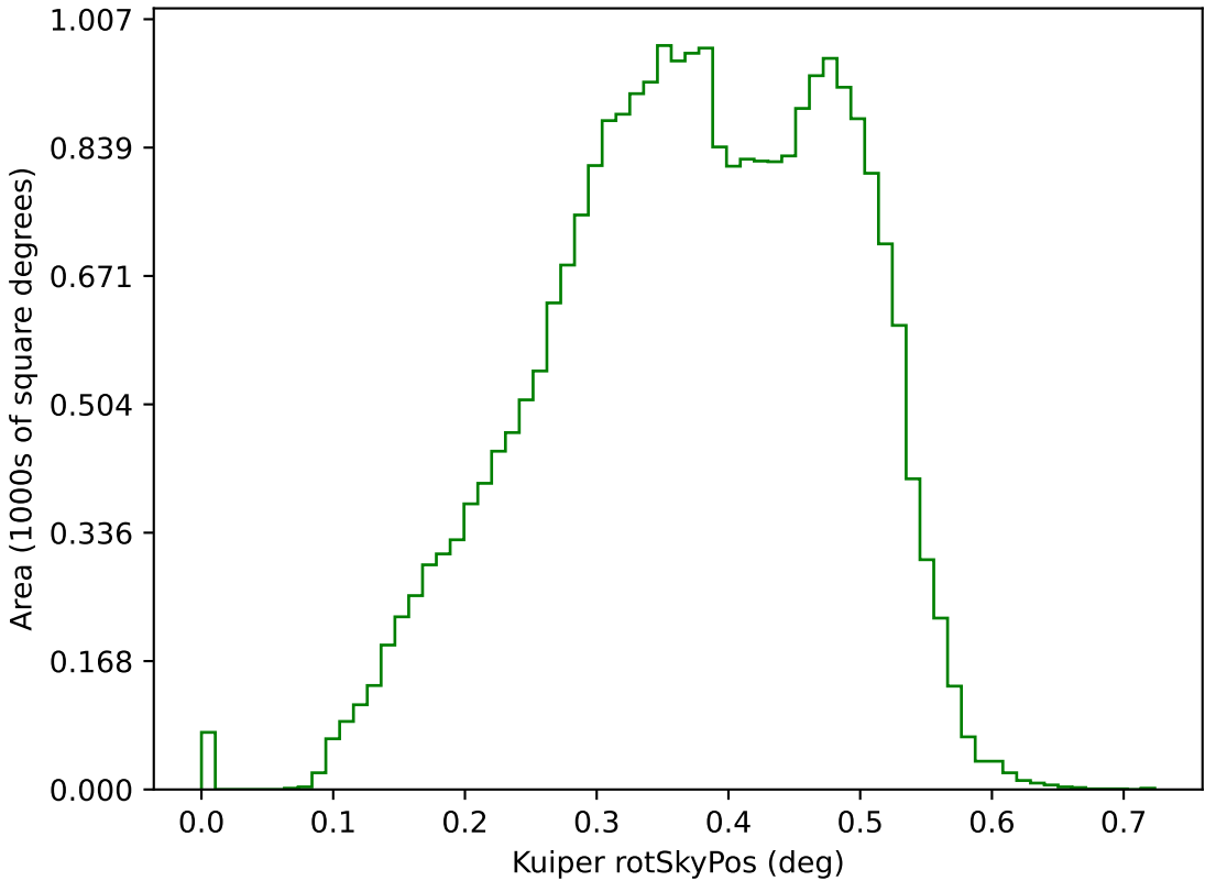
roll_uniform_early_half_mjdp67_v3.4_10yrs g: Kuiper rotSkyPos
