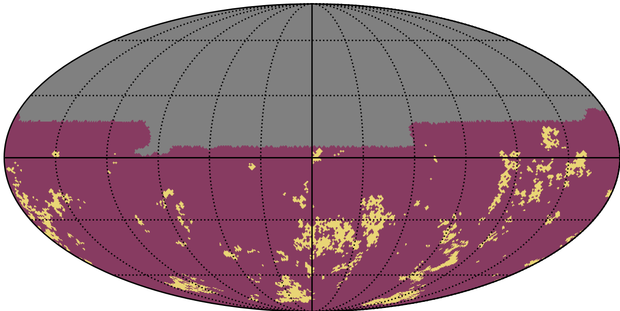
roll_uniform_early_half_mjdp67_v3.4_10yrs u band: Gaps_7hr
