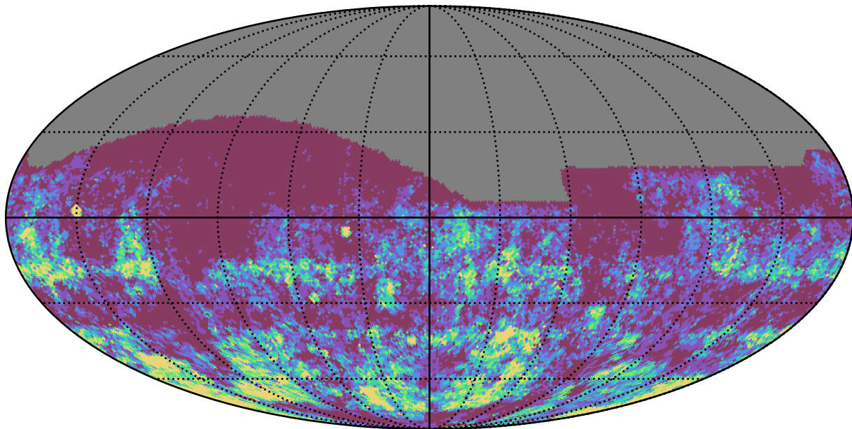
roll_uniform_early_half_mjdp67_v3.4_10yrs r band: Gaps_3hr
