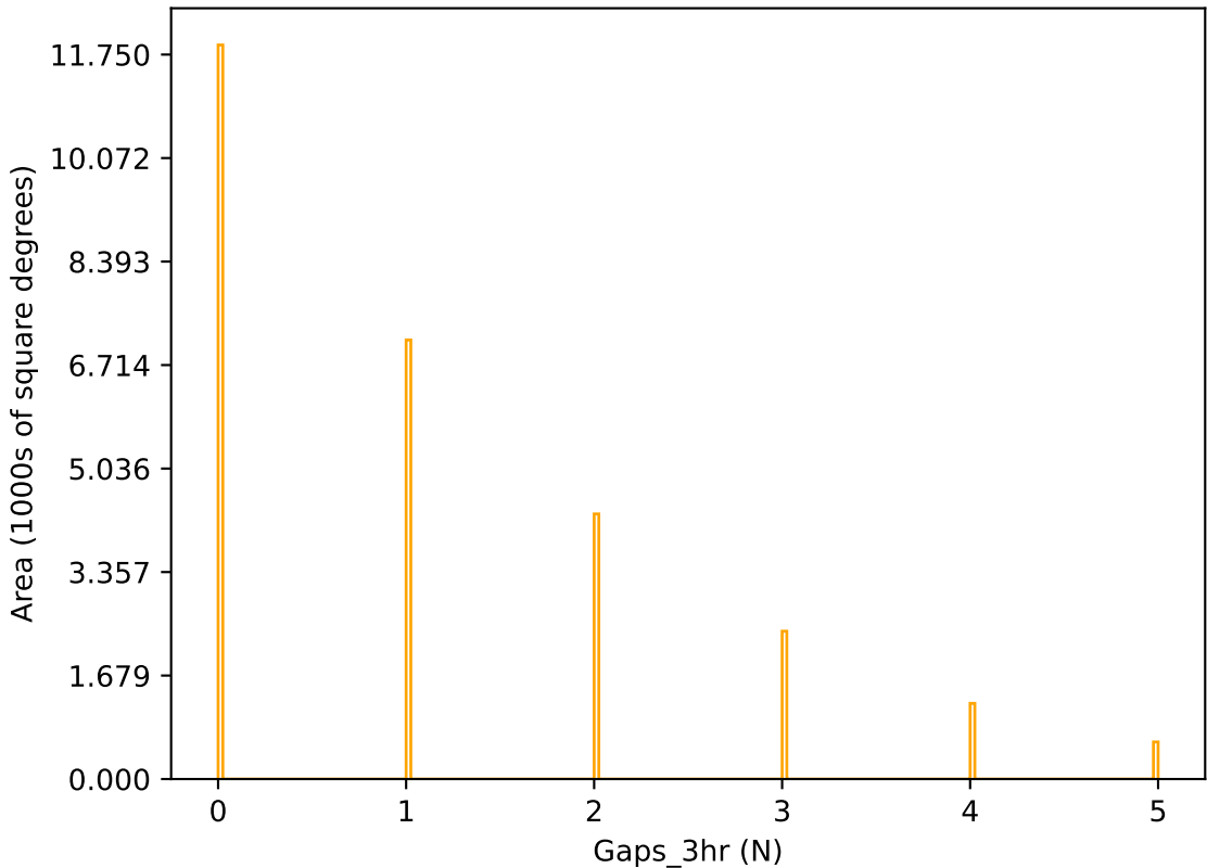
roll_uniform_early_half_mjdp67_v3.4_10yrs r band: Gaps_3hr
