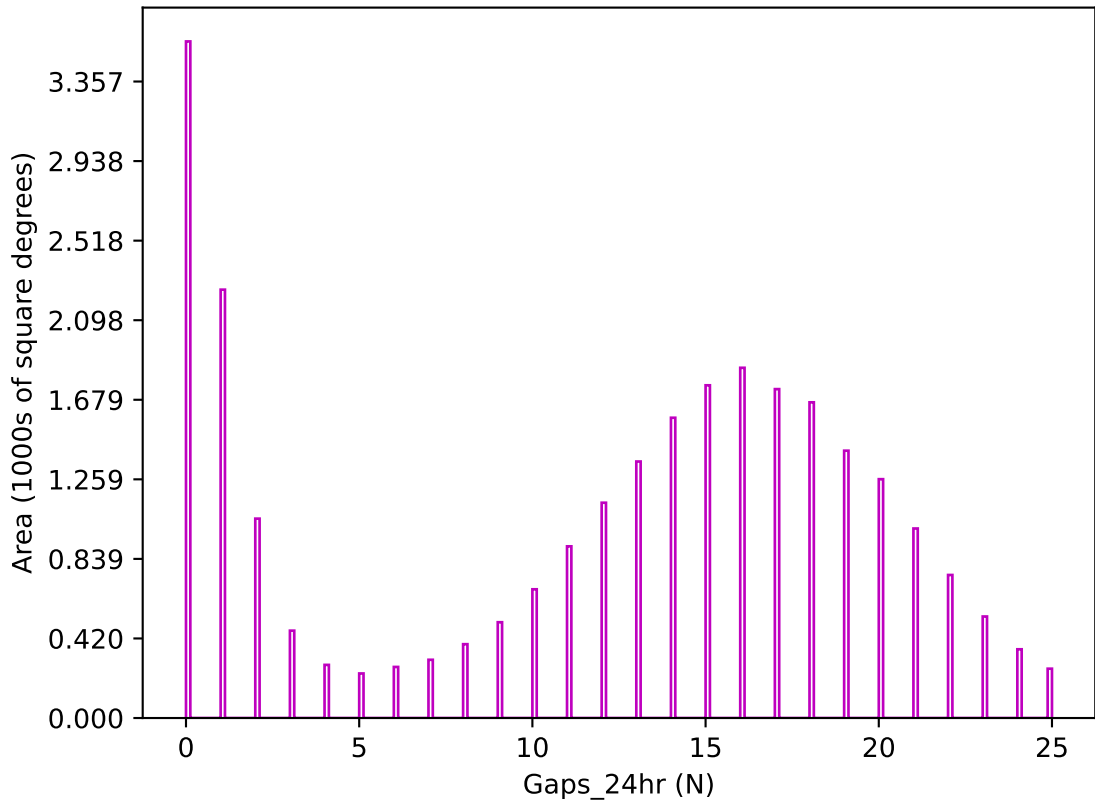
roll_uniform_early_half_mjdp67_v3.4_10yrs z band: Gaps_24hr
