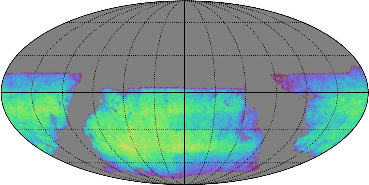
roll_uniform_early_half_mjdp67_v3.4_10yrs i band non-DD year 9: ExgalM5WithCuts
