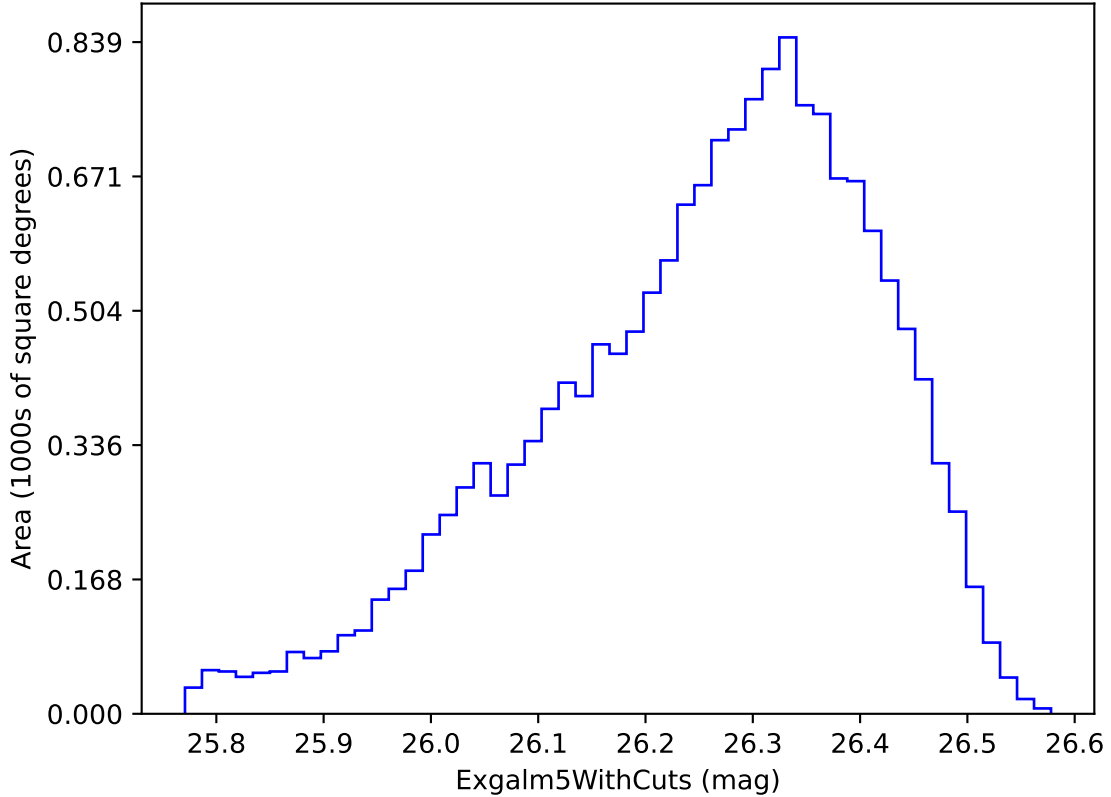
roll_uniform_early_half_mjdp67_v3.4_10yrs i band non-DD year 8: ExgalM5WithCuts
