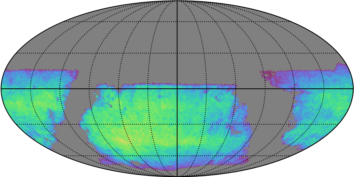
roll_uniform_early_half_mjdp67_v3.4_10yrs i band non-DD year 7: ExgalM5WithCuts
