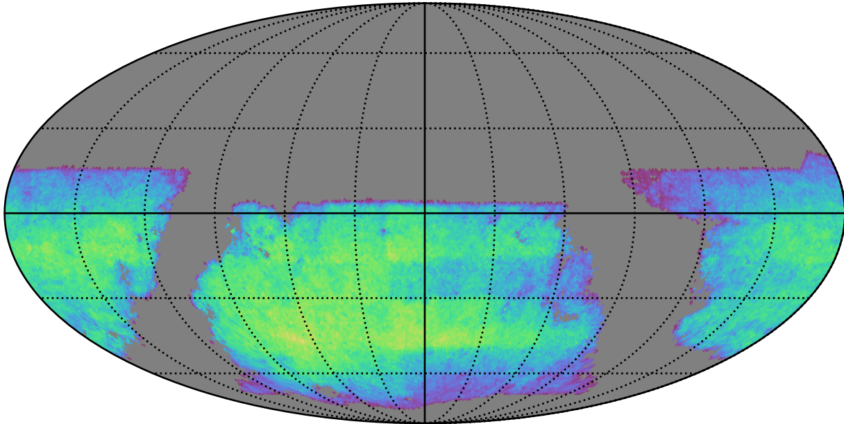
roll_uniform_early_half_mjdp67_v3.4_10yrs i band non-DD year 6: ExgalM5WithCuts
