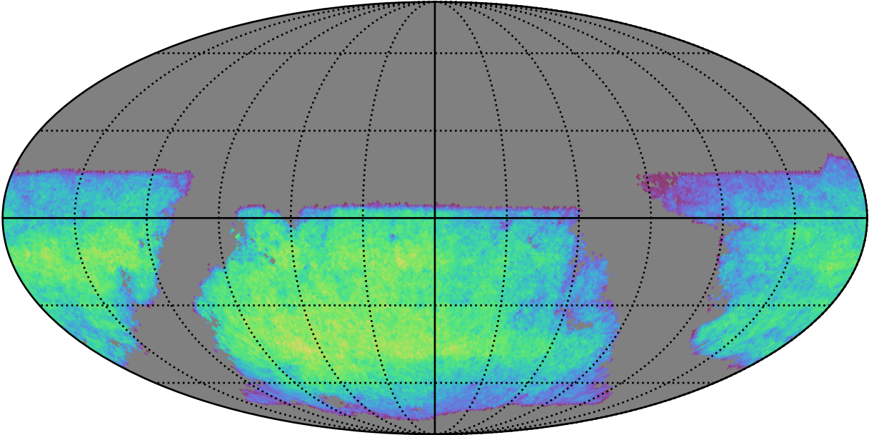
roll_uniform_early_half_mjdp67_v3.4_10yrs i band non-DD year 4: ExgalM5WithCuts
