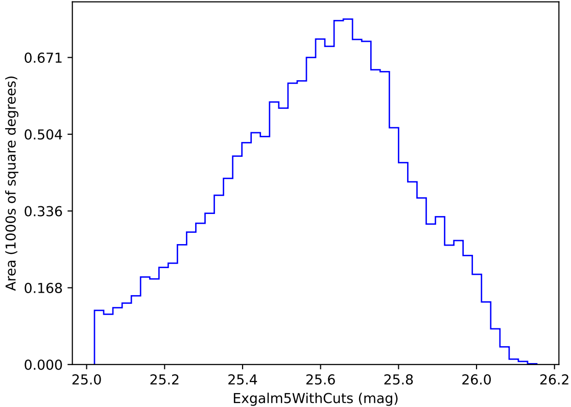
roll_uniform_early_half_mjdp67_v3.4_10yrs i band non-DD year 2: ExgalM5WithCuts
