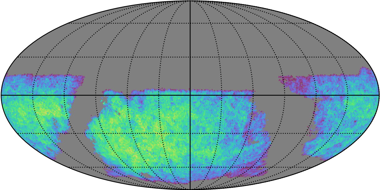
roll_uniform_early_half_mjdp67_v3.4_10yrs i band non-DD year 1: ExgalM5WithCuts
