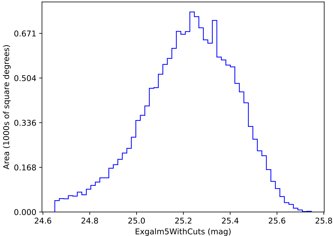
roll_uniform_early_half_mjdp67_v3.4_10yrs i band non-DD year 1: ExgalM5WithCuts
