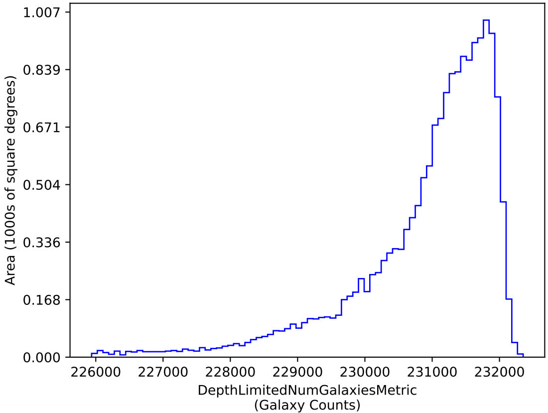
roll_uniform_early_half_mjdp67_v3.4_10yrs i band galaxies non-DD: DepthLimitedNumGalaxiesMetric
