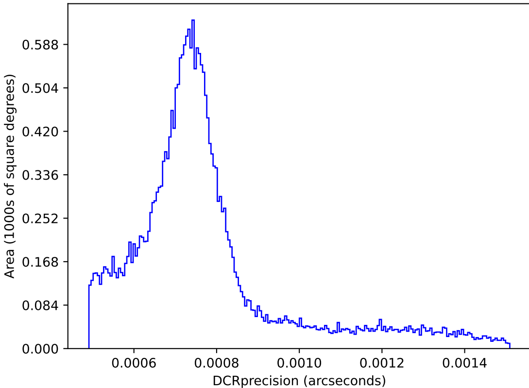
roll_uniform_early_half_mjdp67_v3.4_10yrs : DCRprecision
