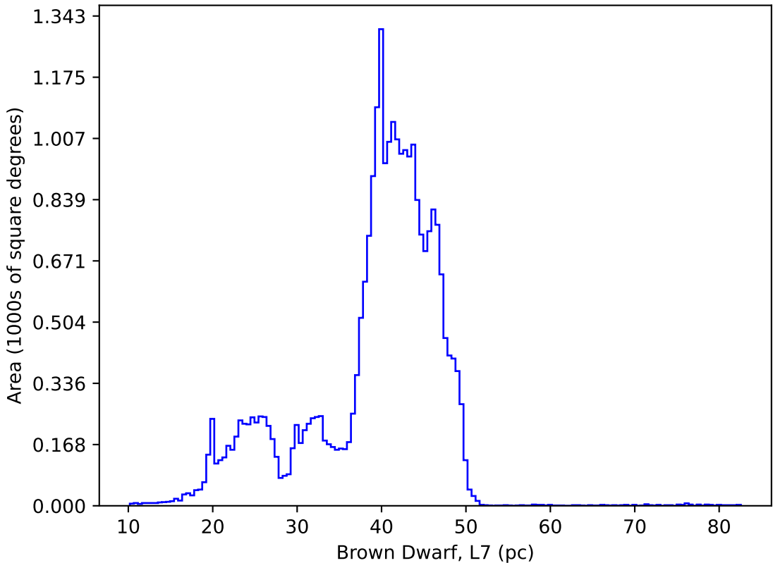
roll_uniform_early_half_mjdp67_v3.4_10yrs : Brown Dwarf, L7
