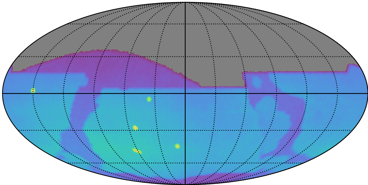
roll_uniform_early_half_mjdp67_v3.4_10yrs : Brown Dwarf, L4
